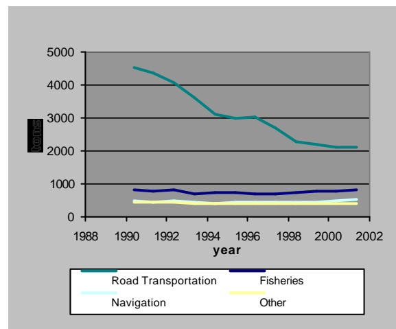
Figure 5.14 Emissions of CO by IPCC sectors on the Faroe Islands. 1990-2001.
