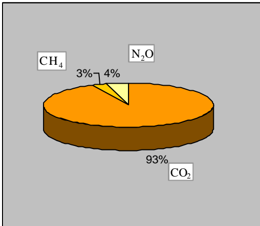
Figure 2.6 Composition of greenhouse gas emissions in the Faroe Islands weighted by GWP values. 2001
