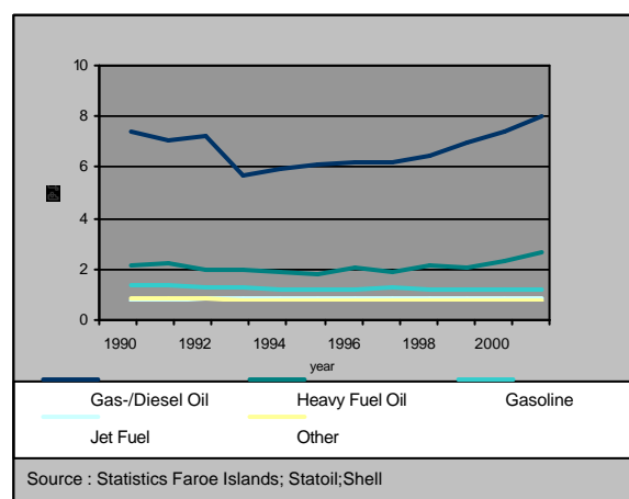
Figure 3.1 Fuel use by fuel type on the Faroe Islands 1990-2001
