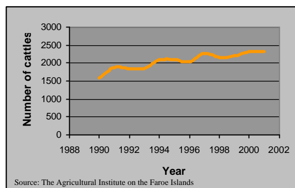
Figure 2.5 Number of cattle's on the Faroe Islands. 1990-2001
