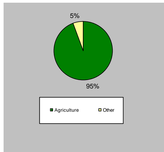
Figure 5.5. Composition of CH 4 emissions by IPCC sectors on the Faroe Islands. 2001
