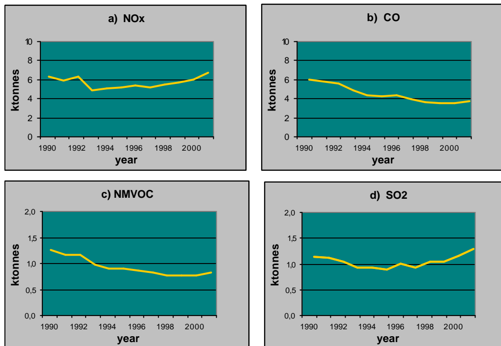
Figure 2.8 Emissions of \text{NO}_x , CO, NMVOC and \text{SO}_2 from 1990-2001.
