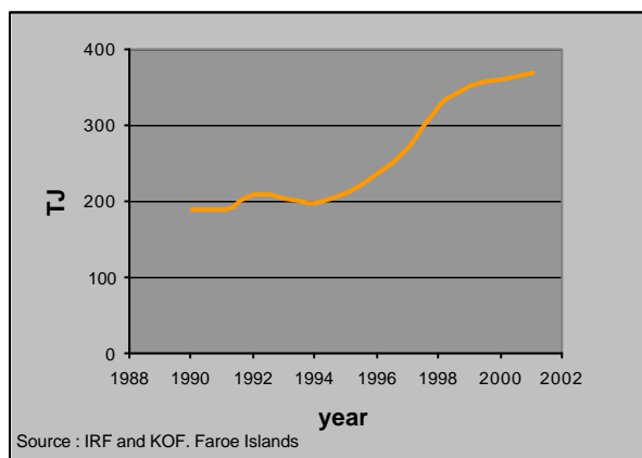
Figure 2.3 Total waste energy on the Faroe Islands. 1990-2001.
