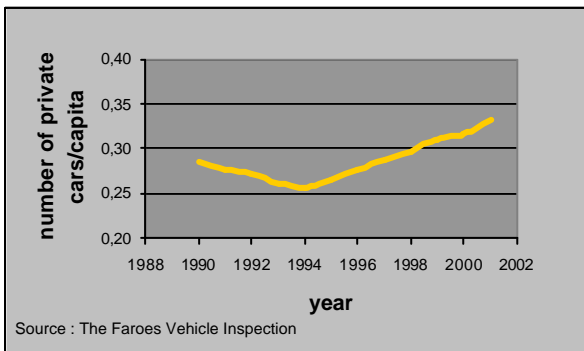
Figure 3.6 Number of private cars/capita on the Faroe Islands. 1990-2001.
