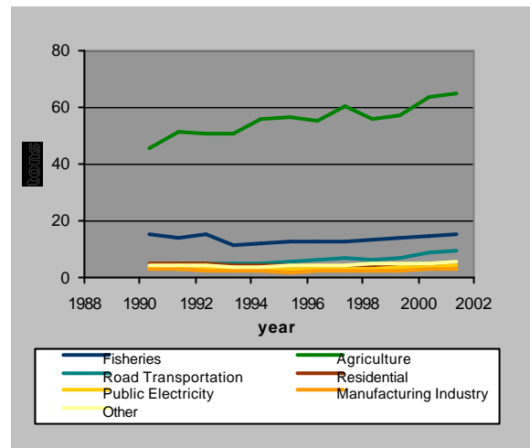
Figure 5.8 Emissions of N 2 O by IPCC sectors on the Faroe Islands. 1990-2001.
