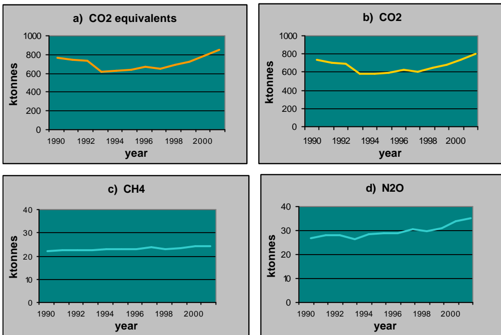
Figure 2.7 Emissions of greenhouse gases from 1990-2001 and derived CO 2 equivalents
