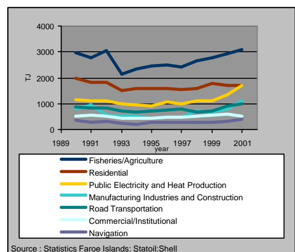
Figure 3.4 Energy use by consumer group in the Faroe Islands 1990-2001
