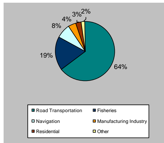
Figure 5.14 Emissions of CO by IPCC sectors on the Faroe Islands. 1990-2001.
