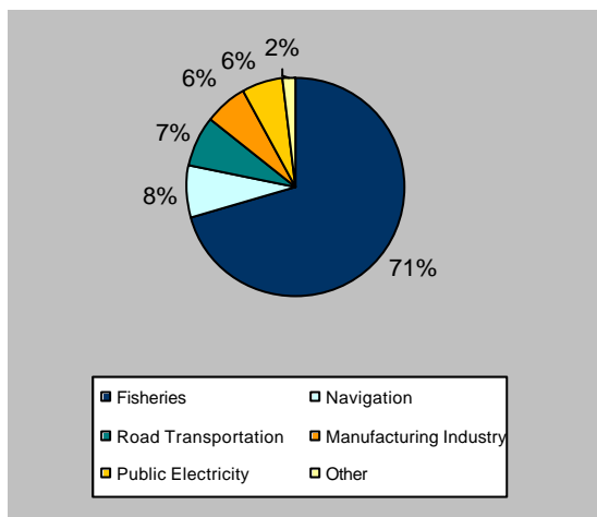
Figure 5.11. Composition of NO x emissions by IPCC sectors on the Faroe Islands. 2001
