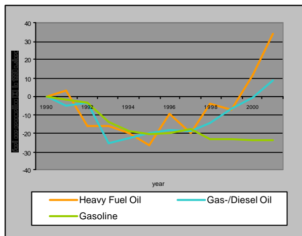
Figure 2.2 The proportion of fuel use compared to 1990 values divided by the type of fuel, 1990-2001.
