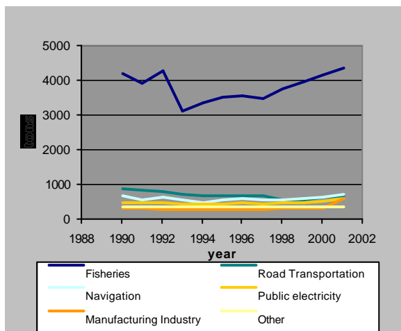
Figure 5.12 Emissions of NO x by IPCC sectors on the Faroe Islands. 1990-2001.
