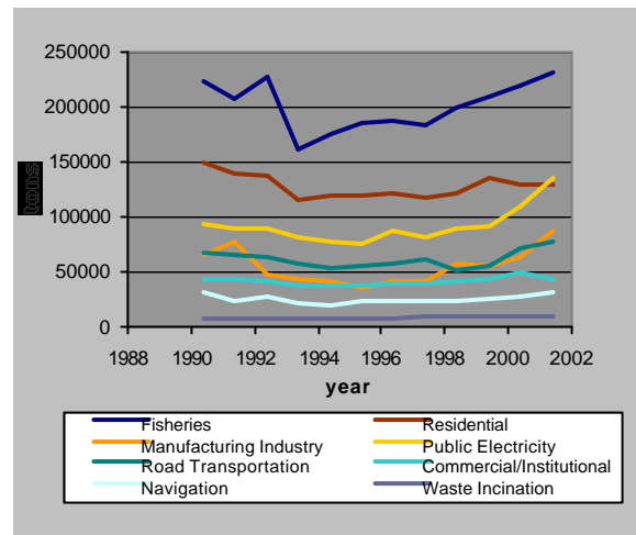
Figure 5.4. Emissions of CO 2 by IPCC sectors in the Faroe Islands. 1990-2001.
