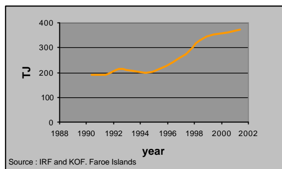
Figure 3.11 Total import to the Faroe Islands. 1990-2001
