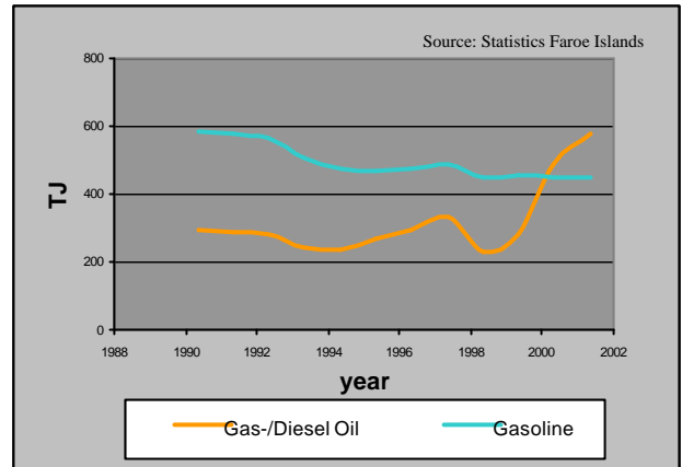
Figure 3.7 Fuel consumption by fuel type for road transportation . 1990-2001.
