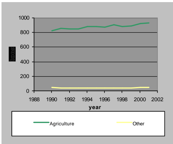
Figure 5.6 Emissions of CH 4 by IPCC sectors on the Faroe Islands. 1990-2001.
