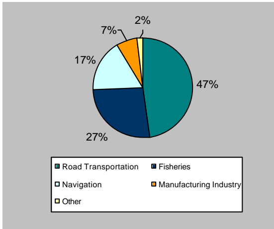
Figure 5.15. Composition of NMVOC emissions by IPCC sectors on the Faroe Islands. 2001
