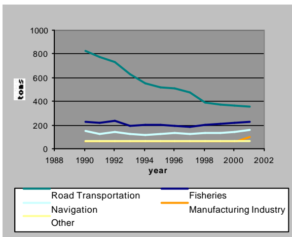
Figure 5.16 Emissions of NMVOC by IPCC sectors on the Faroe Islands. 1990-2001.
