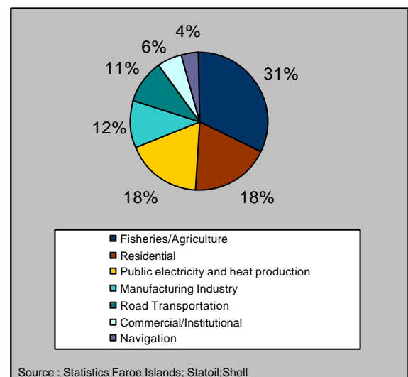
Figure 3.3 Composition of Energy use by consumer group.2001.
