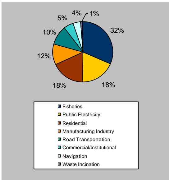
Figure 5.3. Composition of CO 2 emissions by IPCC sectors in the Faroe Islands. 2001.
