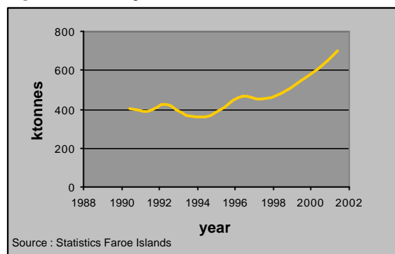
Figure 3.11 Total import to the Faroe Islands. 1990-2001
