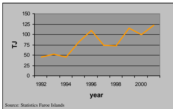
Figure 3.8 Energy use connected to fuel consumption from aviation on the Faroe Islands, 1992-2001.
