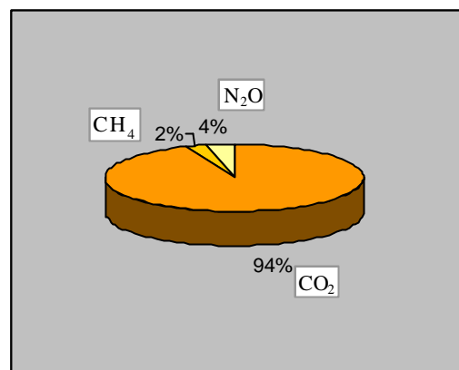
Figure 5.1 Combustion of the greenhouse gases CO 2 , CH 4 and N 2 O weighted by GWP values. 2001
