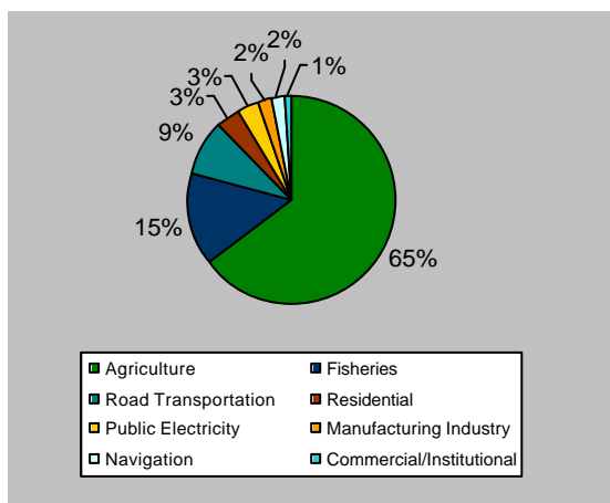
Figure 5.7. Composition of N 2 O emissions by IPCC sectors on the Faroe Islands. 2001.
