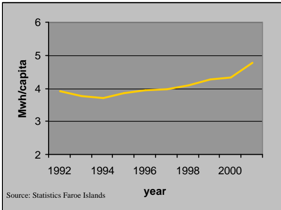
Figure 3.5 Power use (Mwh)/capita in the Faroe Islands. 1990-2001.
