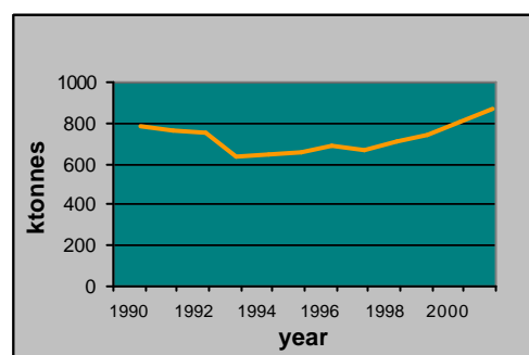
Figure 5.2 Emissions of greenhouse gases in CO 2 equivalents 1990-2001.
