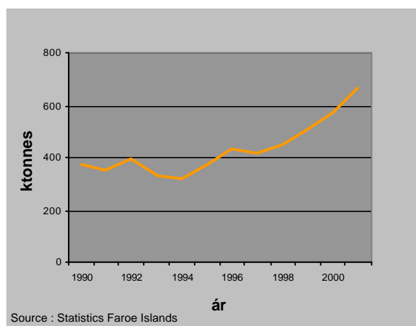
Figure 2.4 Import of goods to the Faroe Islands. 1990-2001.
