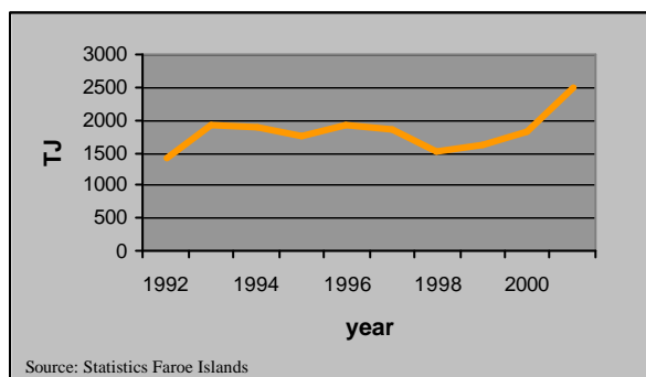
Figure 3.9 Energy use connected to fuel consumption from marine (International bunkers) in the Faroe Islands. 1990-2001.
