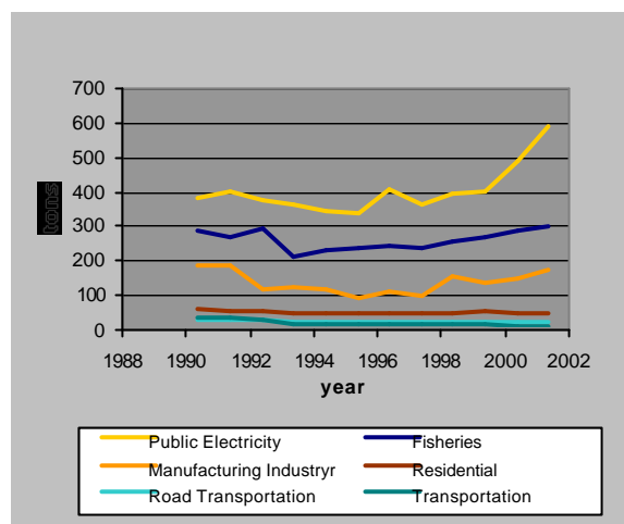
Figure 5.10 Emissions of SO 2 by IPCC sectors on the Faroe Islands. 1990-2001.
