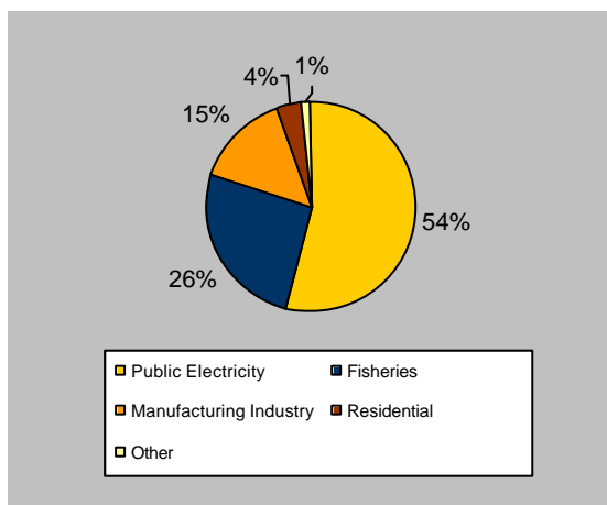
Figure 5.9. Composition of SO 2 emissions by IPCC sectors on the Faroe Islands. 2001
