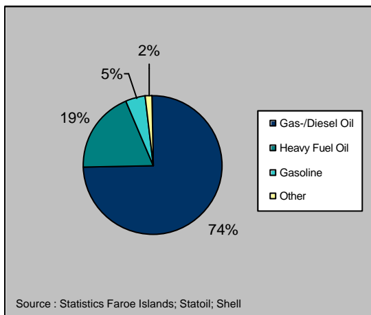
Figure 3.2 Composition of fuel types on the Faroe Islands. 2001.
